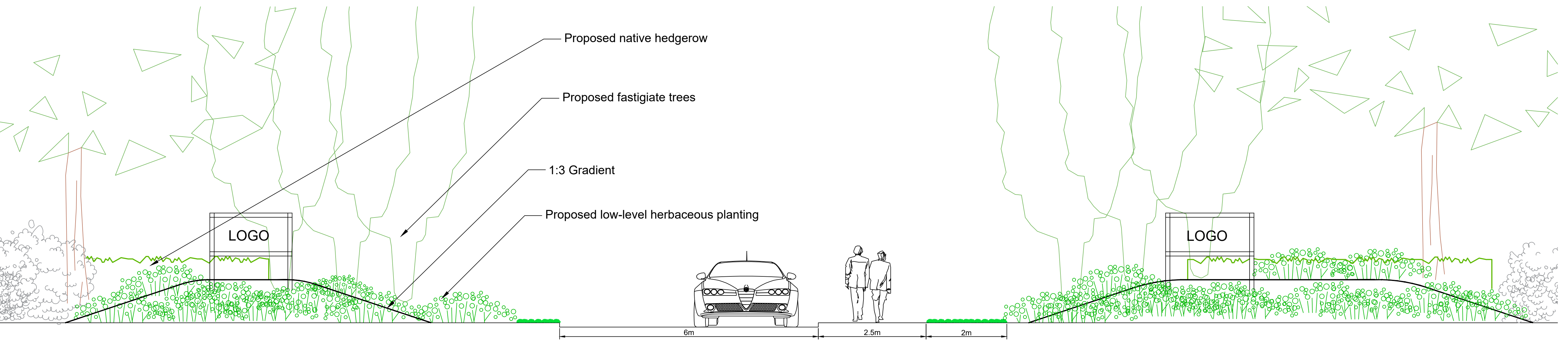
A 2 Scale 1:50 - Cross-section Section from A259, Grevatt's Lane facing south towards new golf course access road
