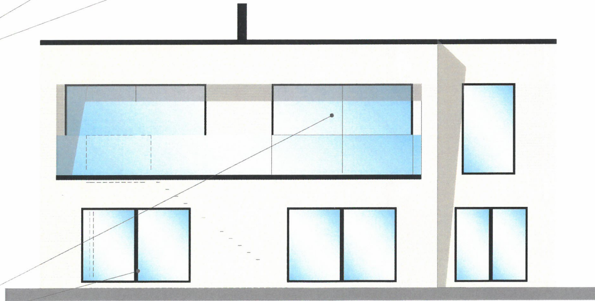
REAR ELEVATION
