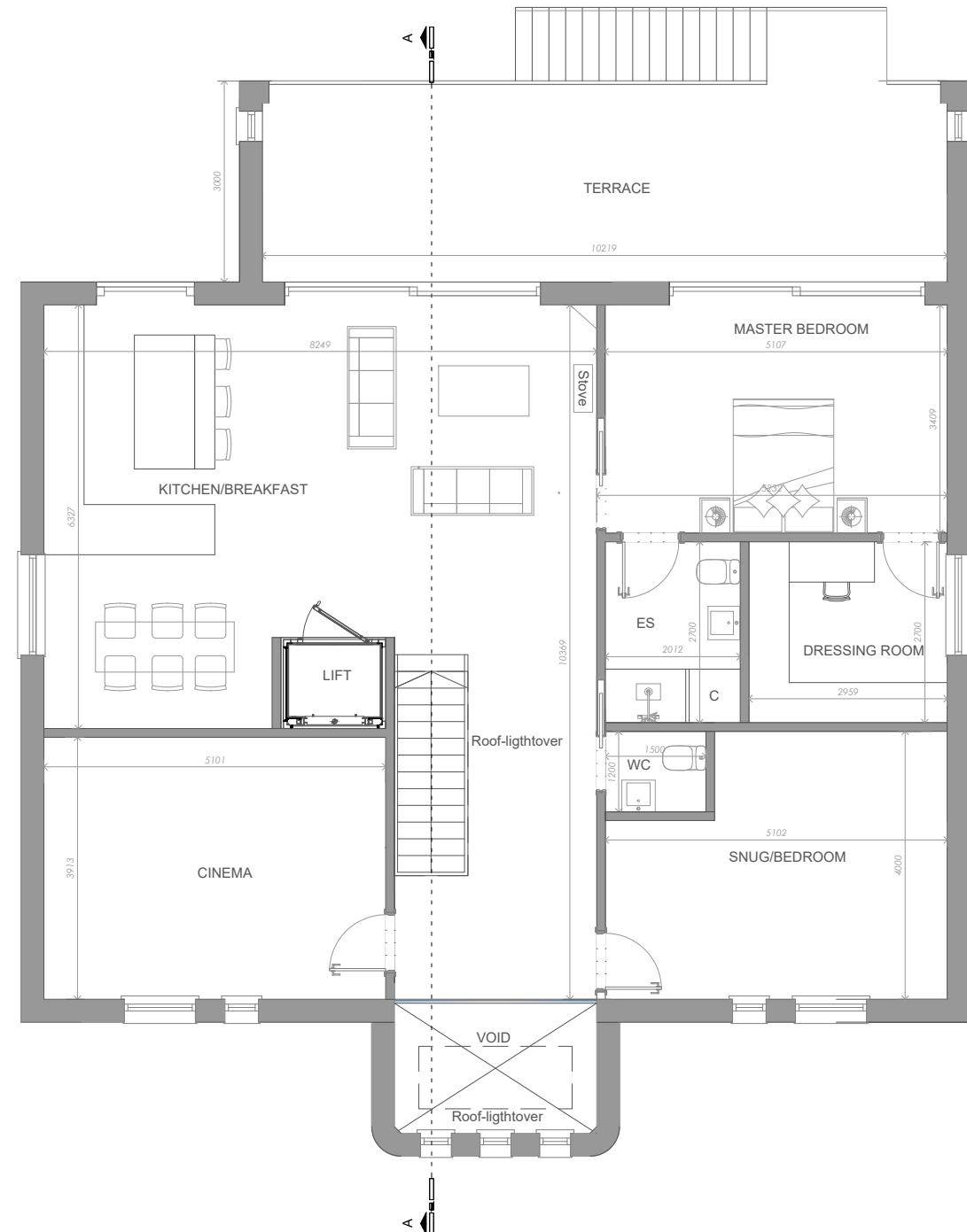
FIRST FLOOR GIA 150m 2
