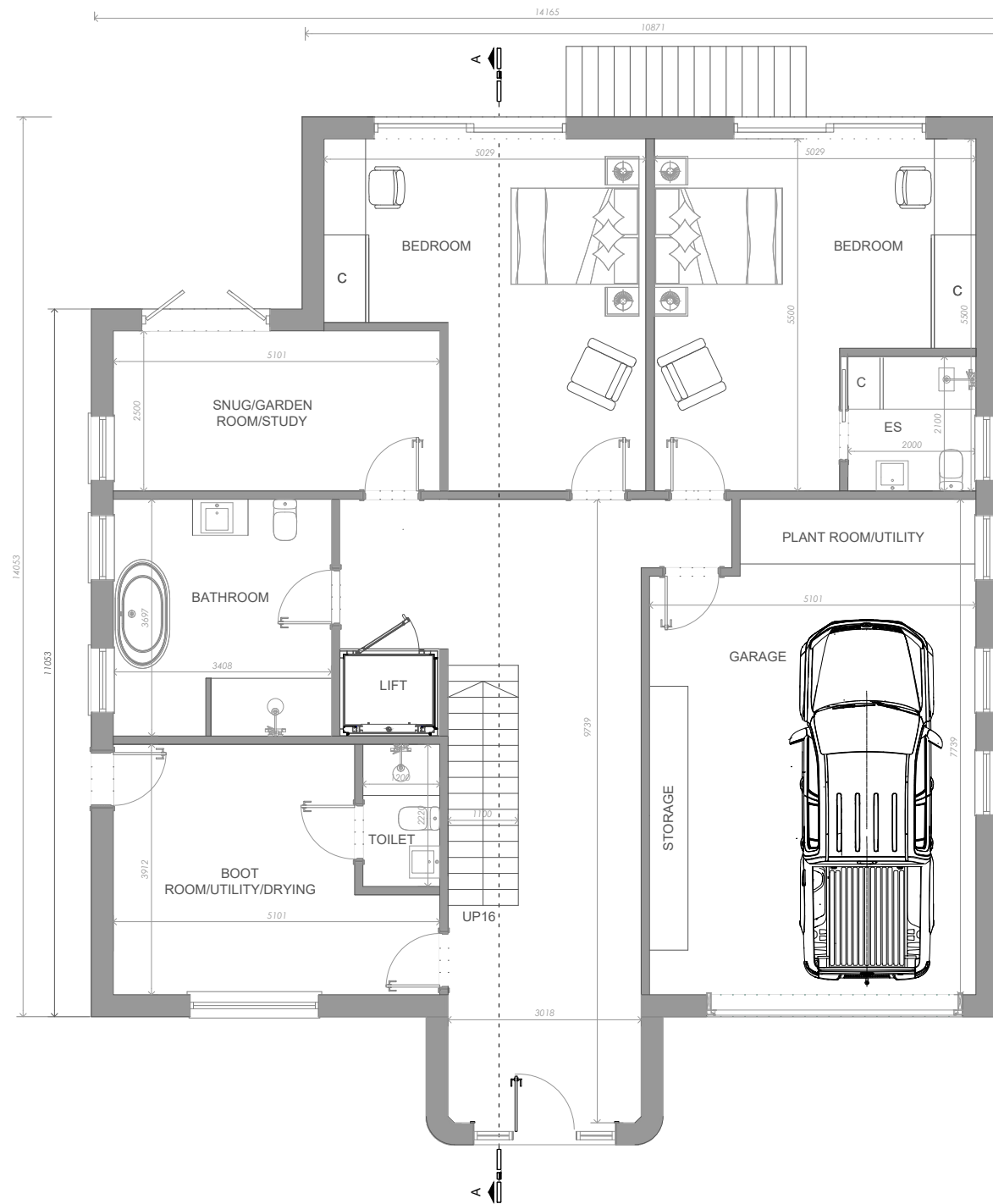
GROUND FLOOR GIA 176m 2
