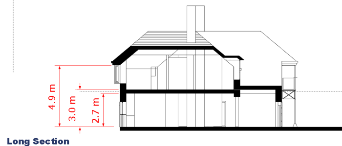
Long Section
