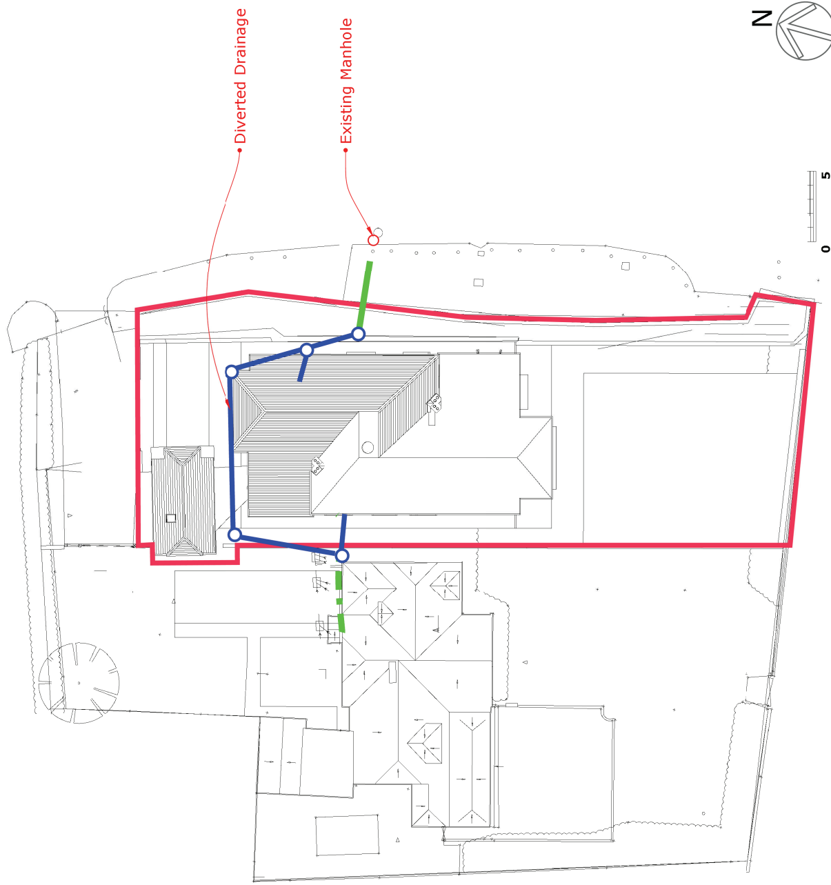
Drainage diversions 1:250 @a3 (Indicative)
