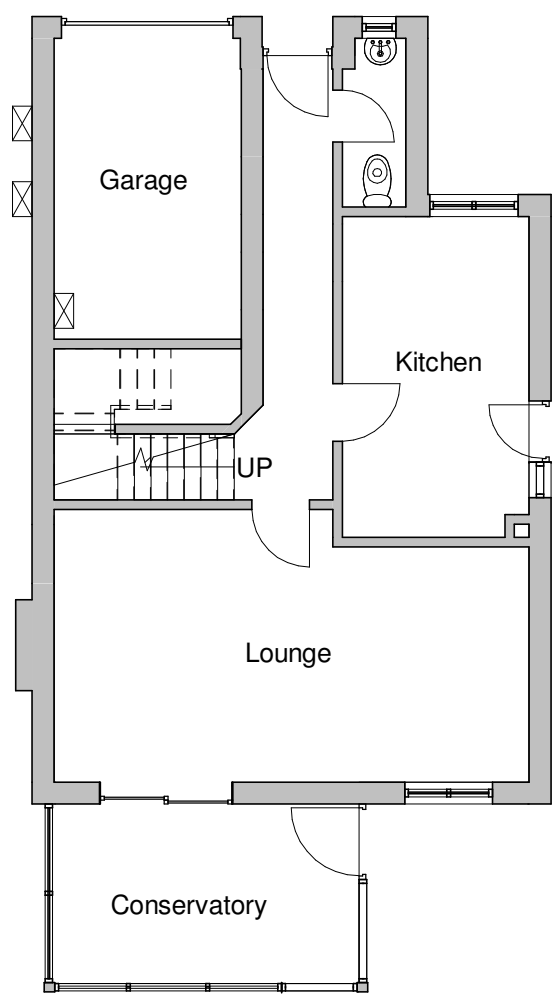
Existing Ground Floor 1 : 100
