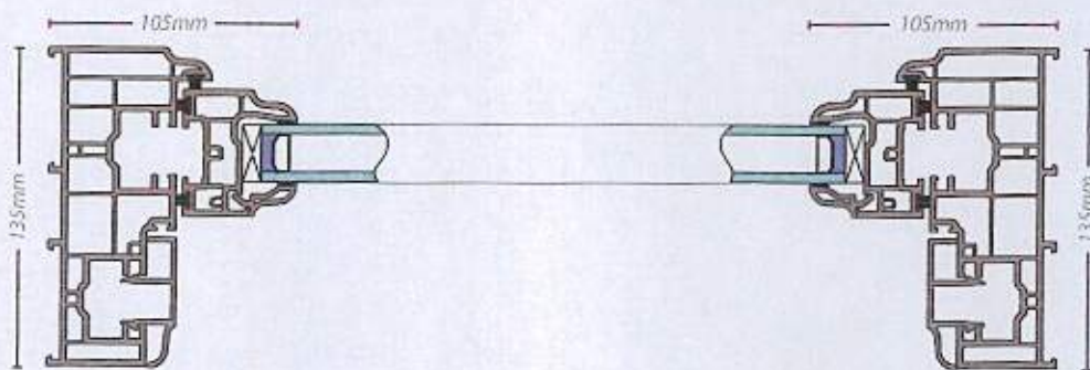
Horizontal section through top sash
