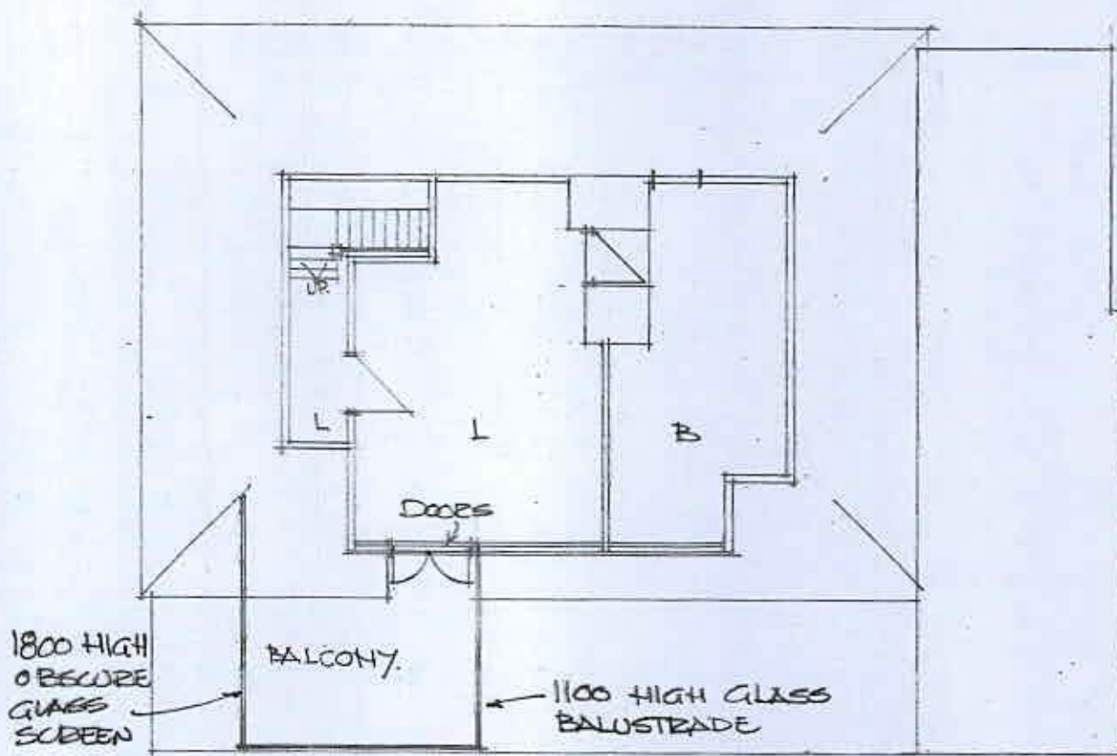
FIRST FLOOR PLAN PROPOSED. ALTERATIONS AND EXTENSIONS TO 24 WEST DRIVE ELMER
