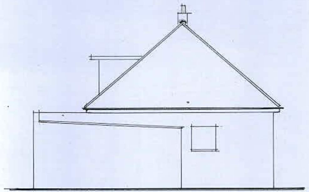
SIDE ELEVATION - NORTH - 1-100.
