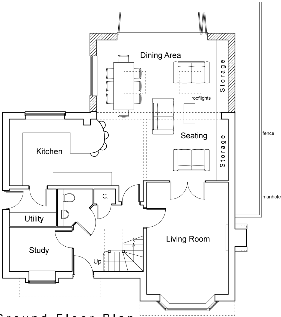
Ground Floor Plan Option One
