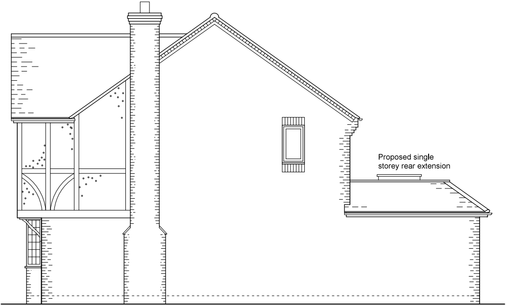
East Elevation
