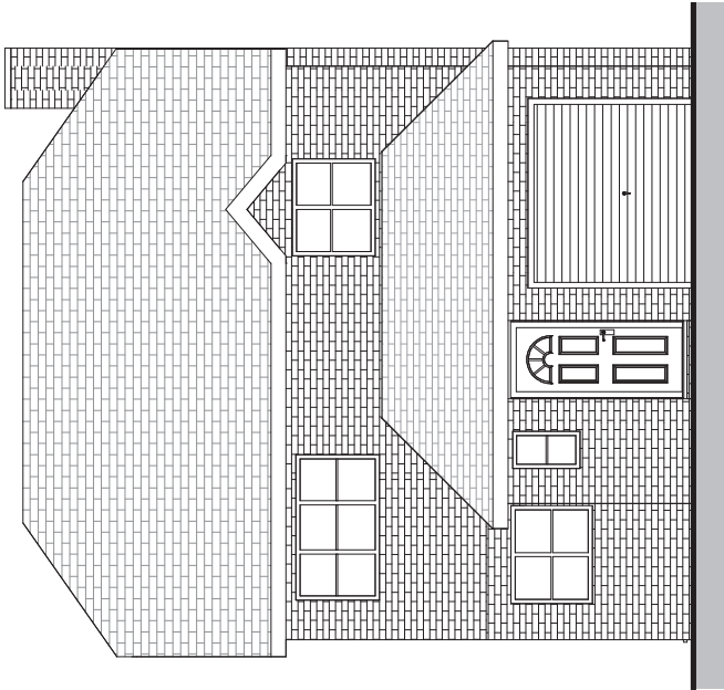
Existing North Elevation 1 : 100
