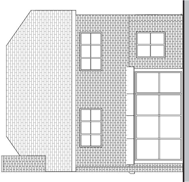
Existing South Elevation 1 : 100
