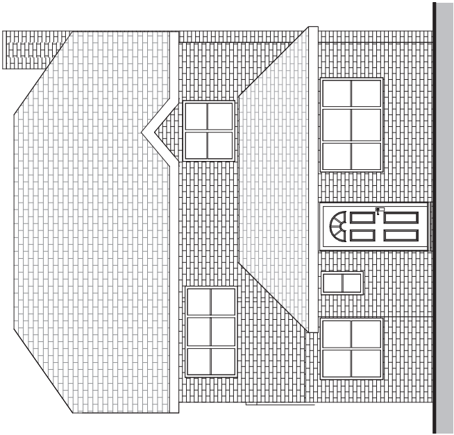
Proposed North Elevation 1 : 100
