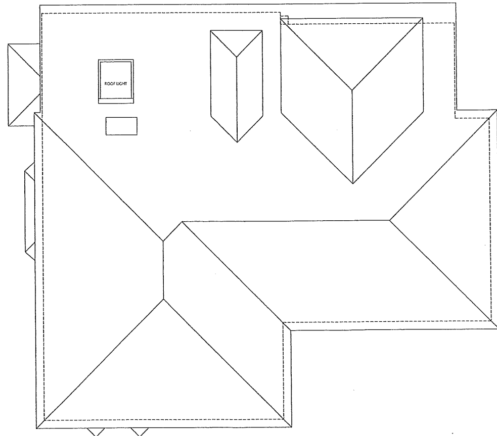
Roof Plan
