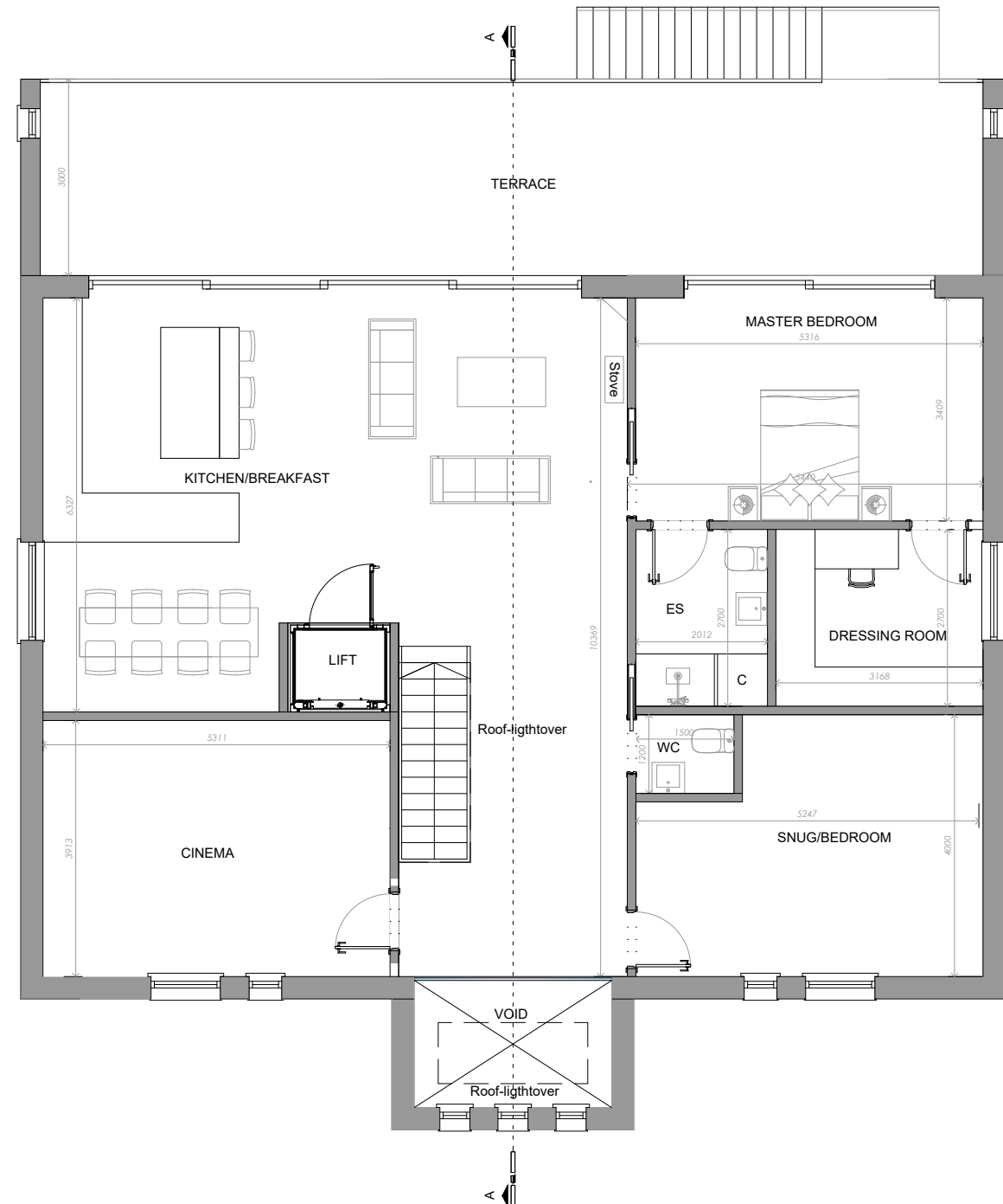
FIRST FLOOR GIA 150m²
