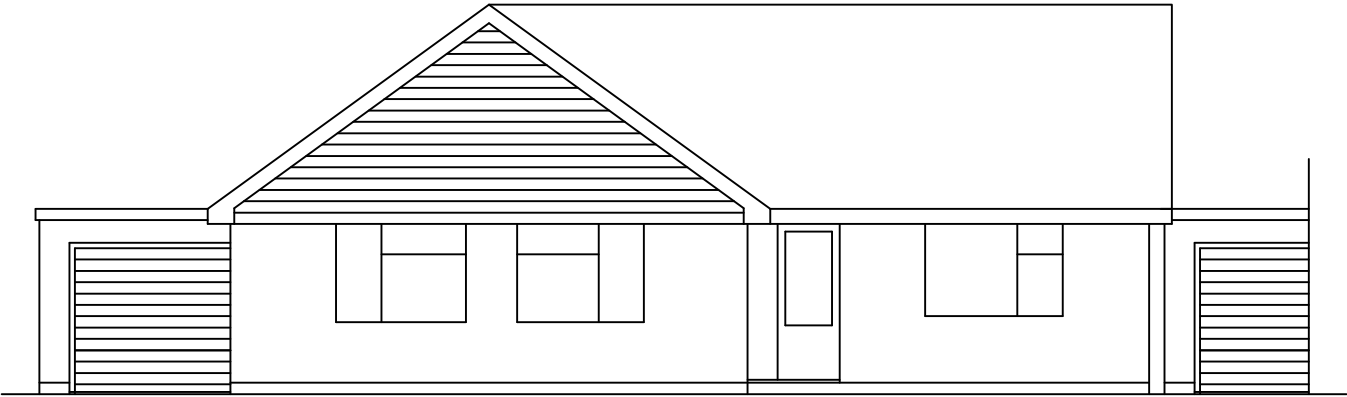
Existing Front Elevation (West)
