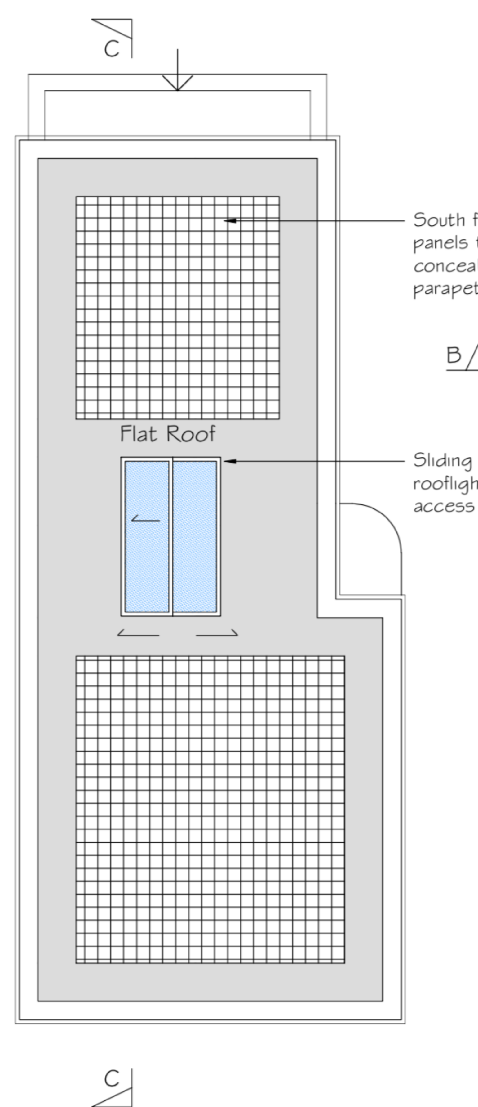
PROPOSED ROOF PLAN @ 1:100
