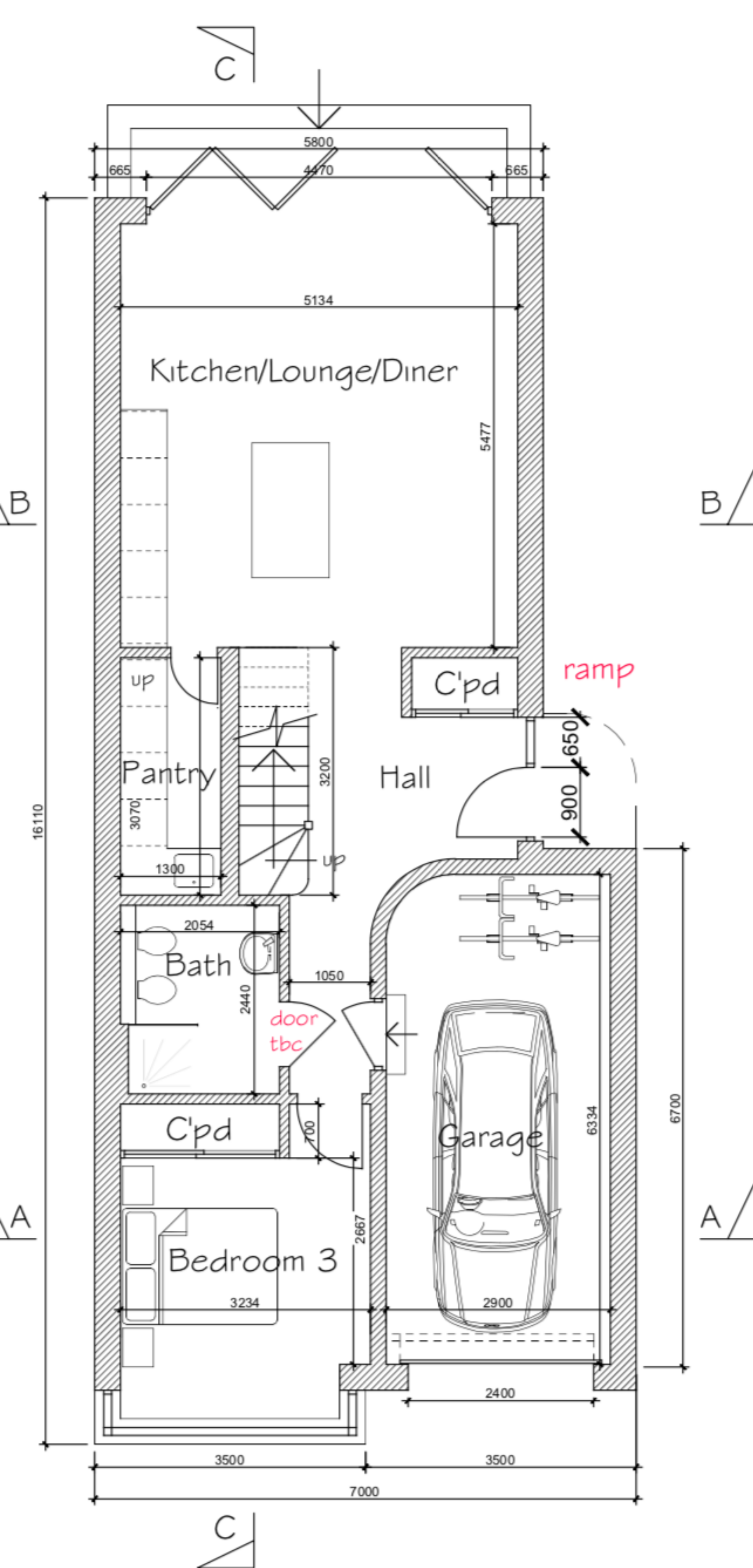
PROPOSED GROUND FLOOR PLAN @ 1:100
