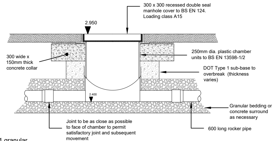
Shallow Foul Access Chamber Detail Type 4 (for use in internal areas)
