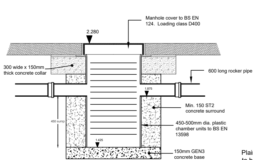
Shallow Silt Trap Inspection Chamber Detail (for use in areas subject to vehicular traffic)
