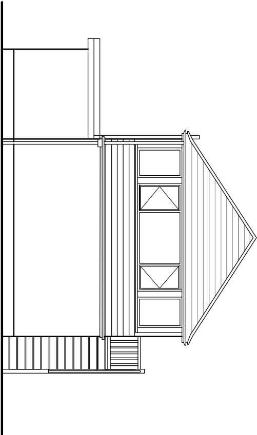
EXISTING REAR (SOUTH) ELEVATION
