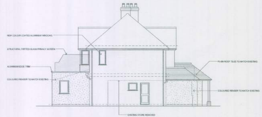
SIDE (EAST) ELEVATION
