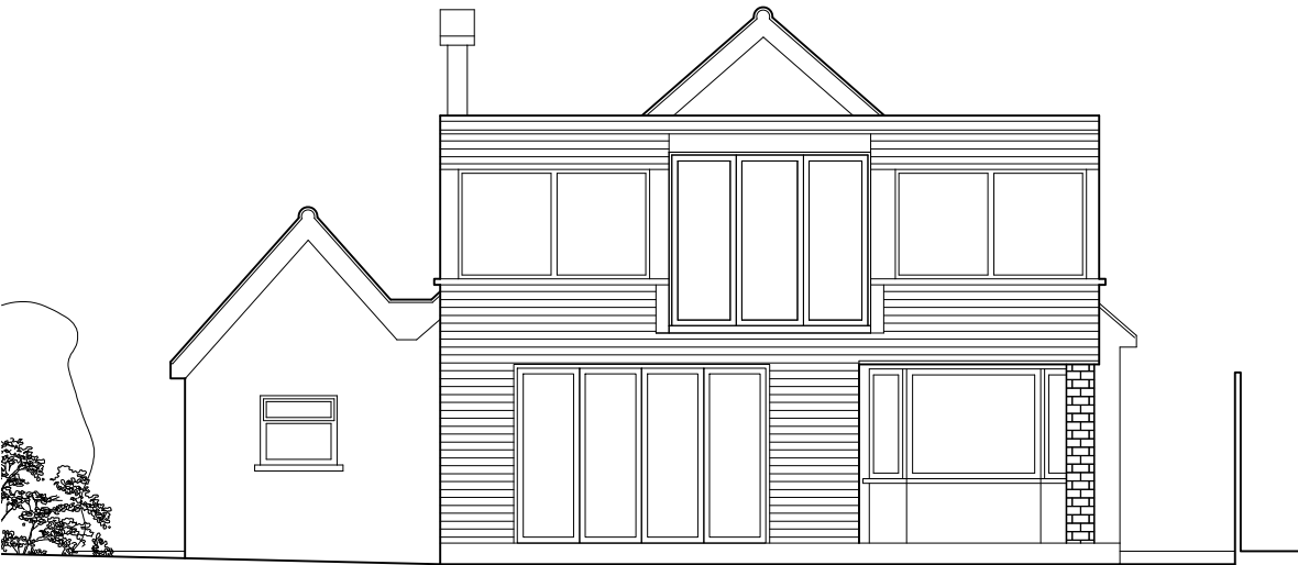
+EL South elevation - scale 1:50
