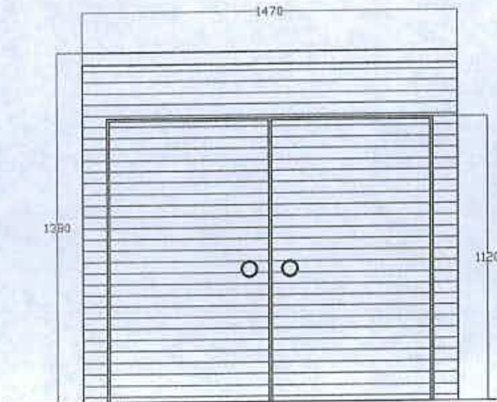
FRONT ELEVATION
