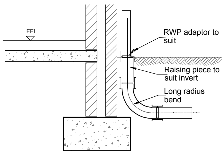
RWP DETAIL
