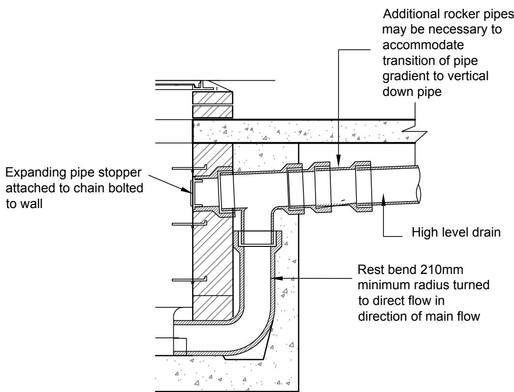
BACKDROP TO EXISTING MANHOLE
