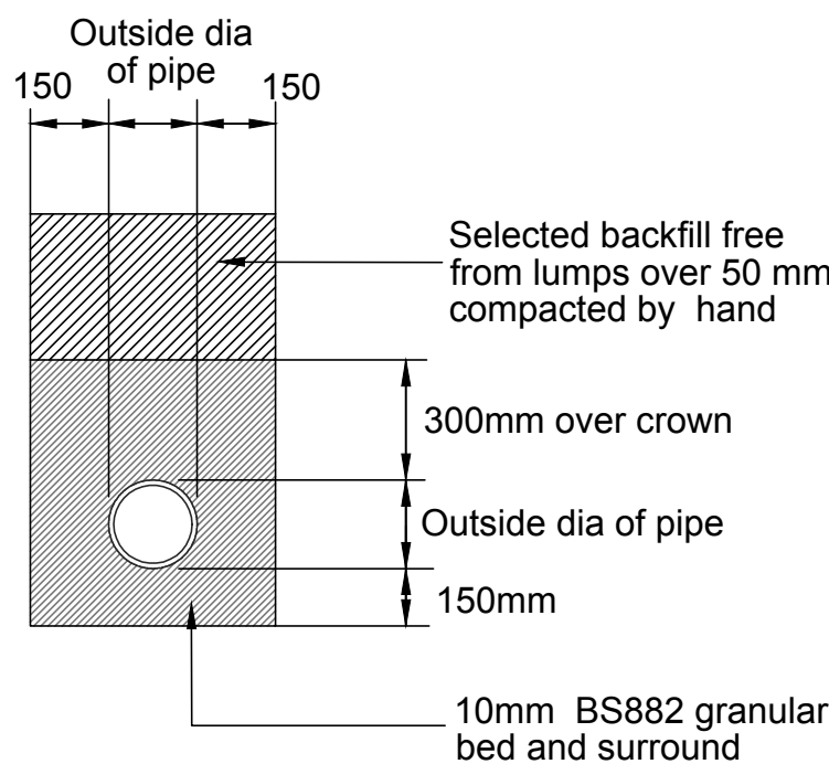
BEDDING CLASS S
