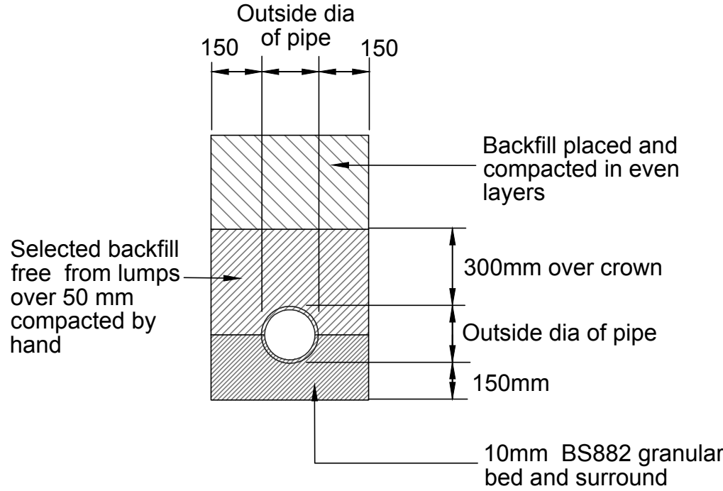
BEDDING CLASS B
