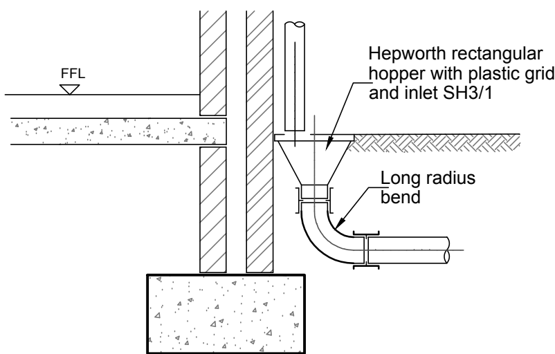
RWP WITH ACCESS DETAIL
