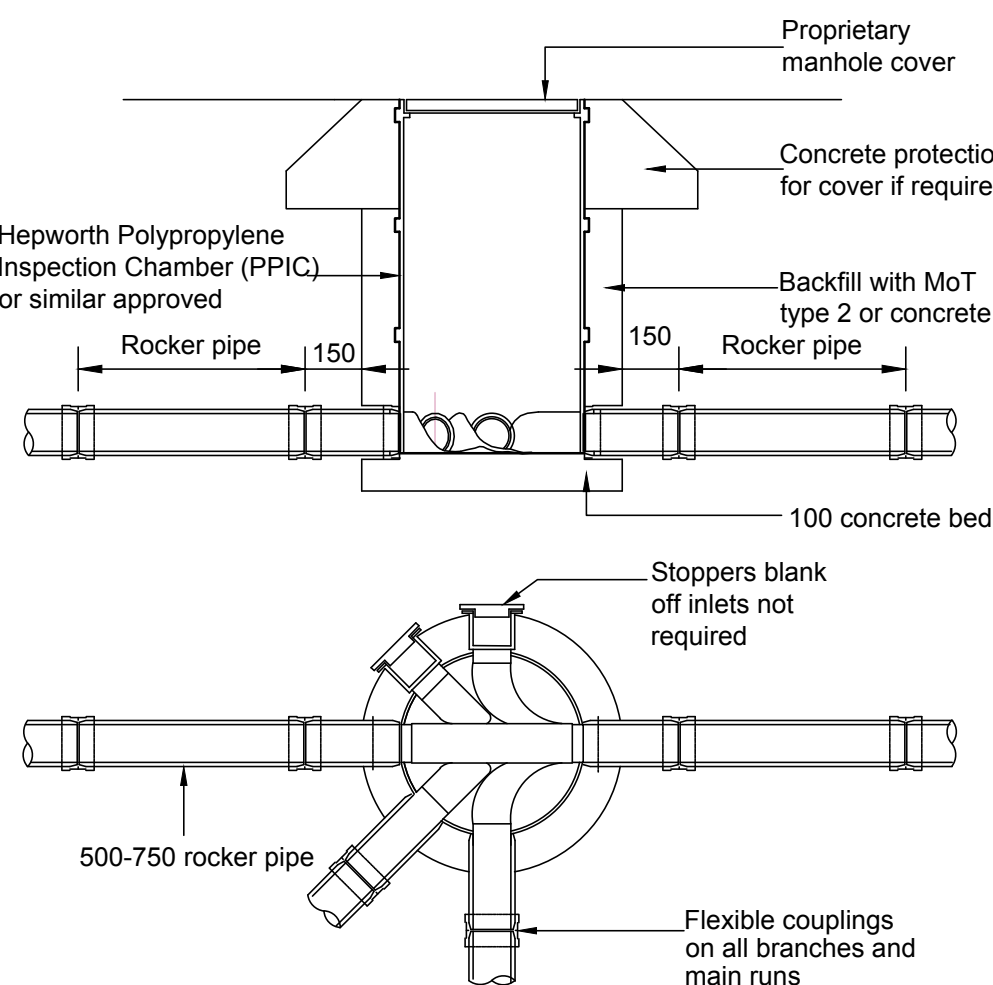
POLYPROPYLENE INSPECTION CHAMBER (MANHOLE TYPE Z)
