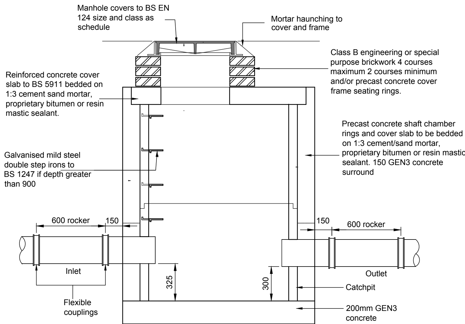
SW CATCHPIT PCC MANHOLE
