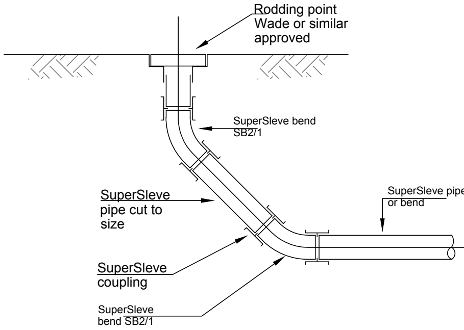
RODDING EYE DETAIL
