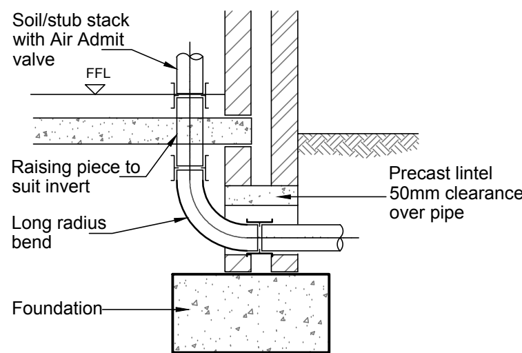
STUB STACK/SVP DETAIL
