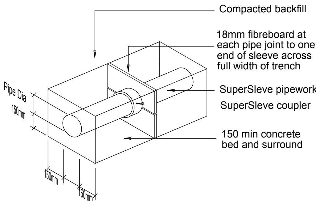
CONCRETE BED AND SURROUND FOR DRAINS WITH LESS THAN 1200mm COVER FROM TOP OF BARREL TO FINISHED ROAD LEVEL
