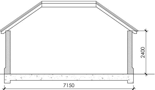
PROPOSED ELEVATION BB 1:100
