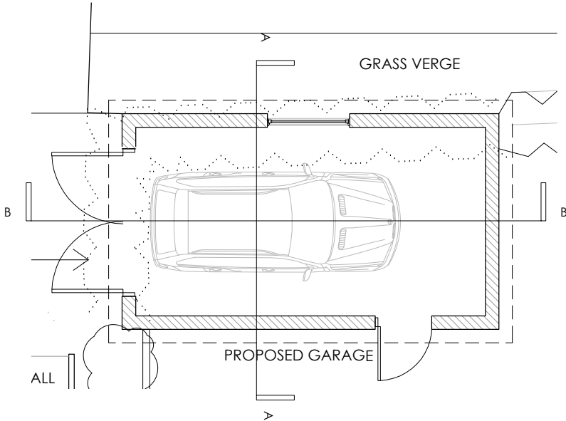
PROPOSED GARAGE PLAN 1:100
