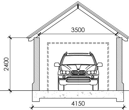
PROPOSED ELEVATION AA 1:100
