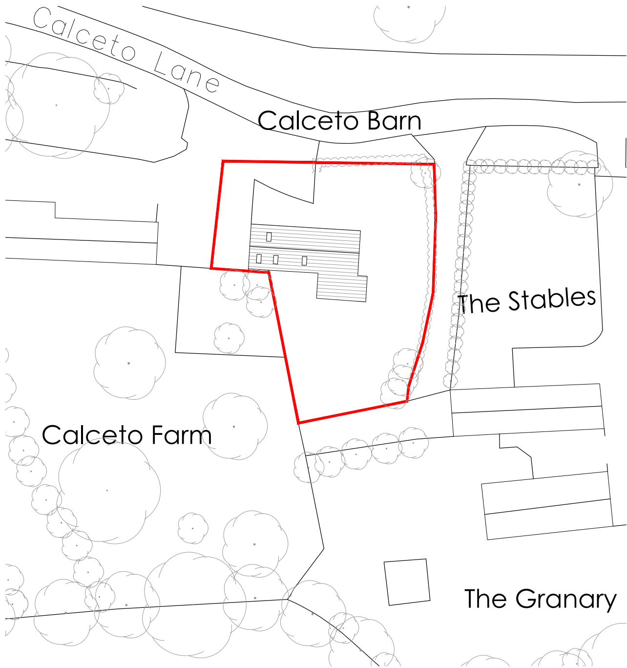
BLOCK PLAN 1:500
