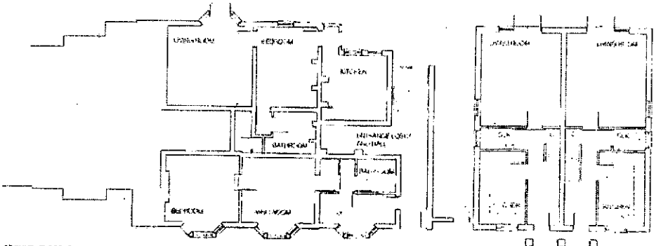
GROUND FLOOR PLAN - AS PROPOSED 1:100 @ A1
