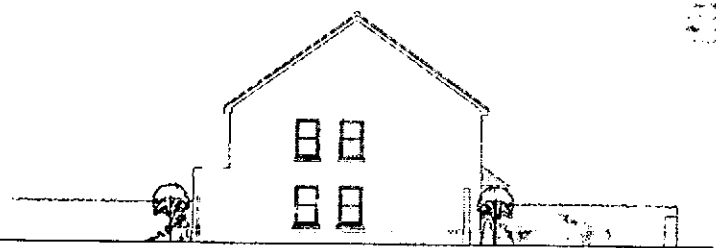
EAST ELEVATION - AS PROPOSED
