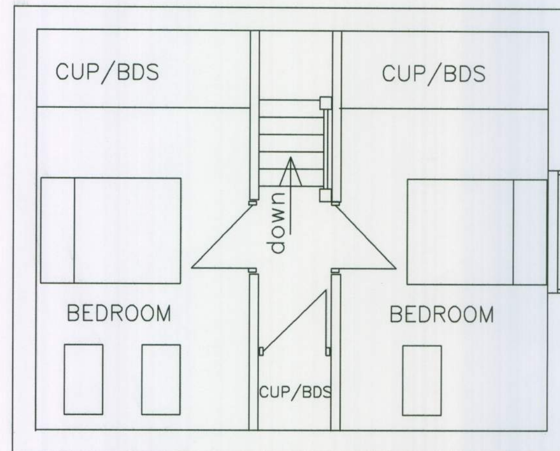
PROPOSED FIRST FLOOR SCALE 1-50
