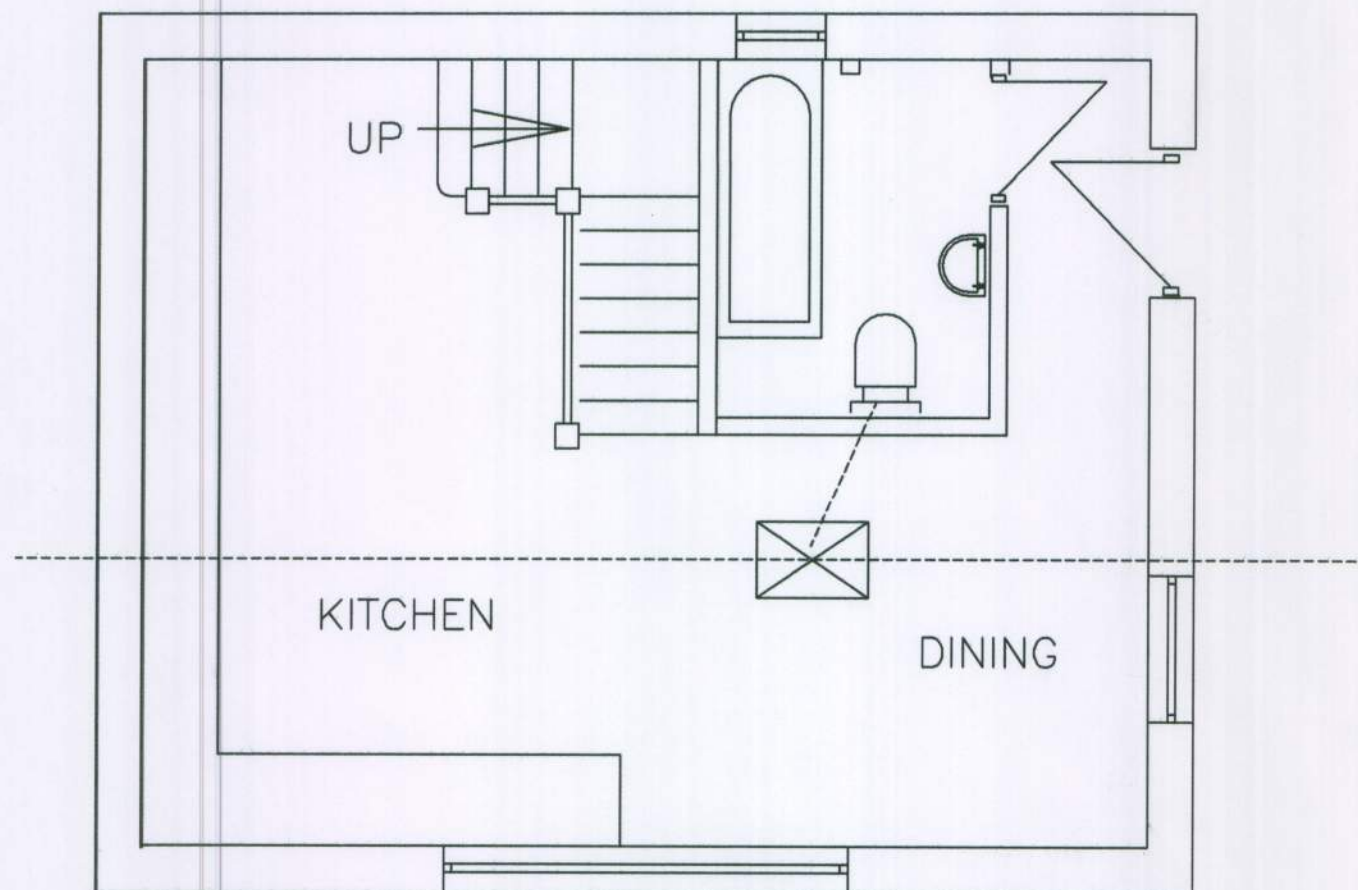
PROPOSED GROUND FLOOR SCALE 1-50
