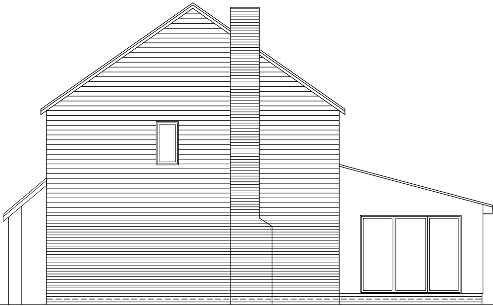
Proposed Side Elevation (South) 1:100
