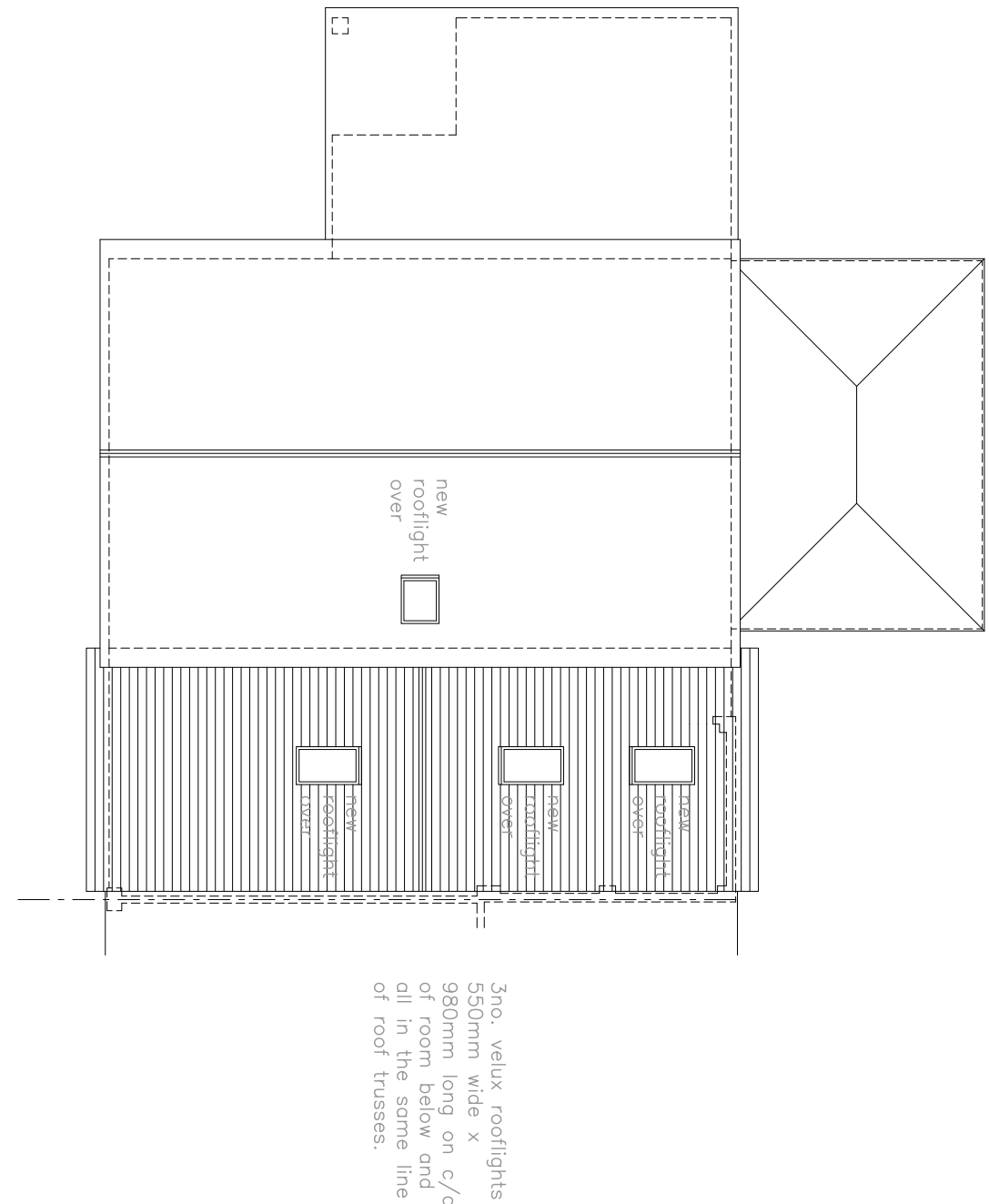
ROOF PLAN 1/100
