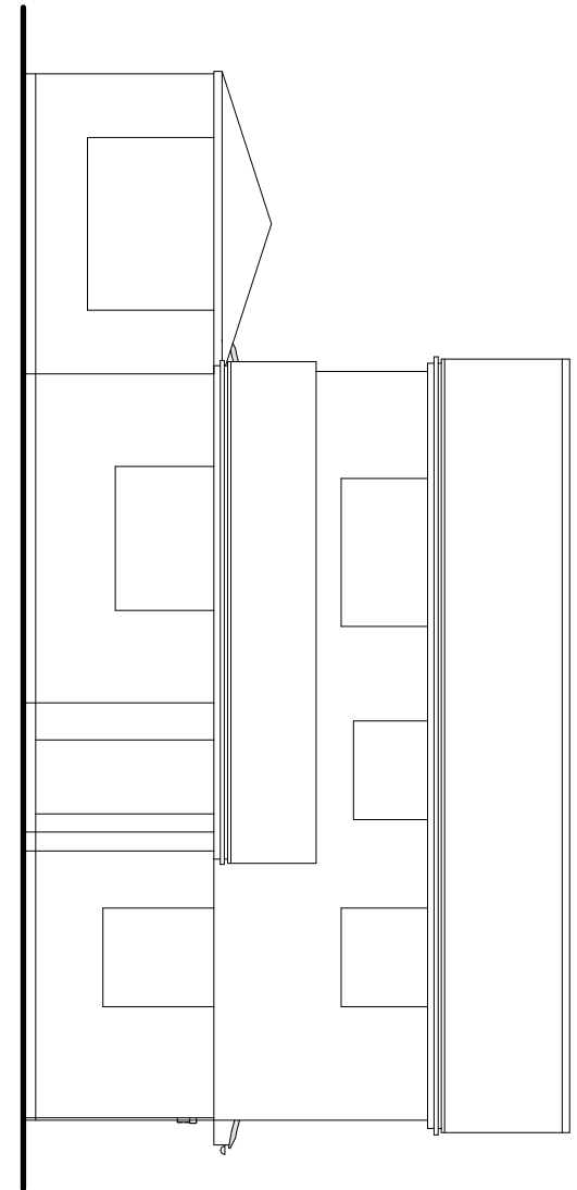
SOUTH ELEVATION 1/100
