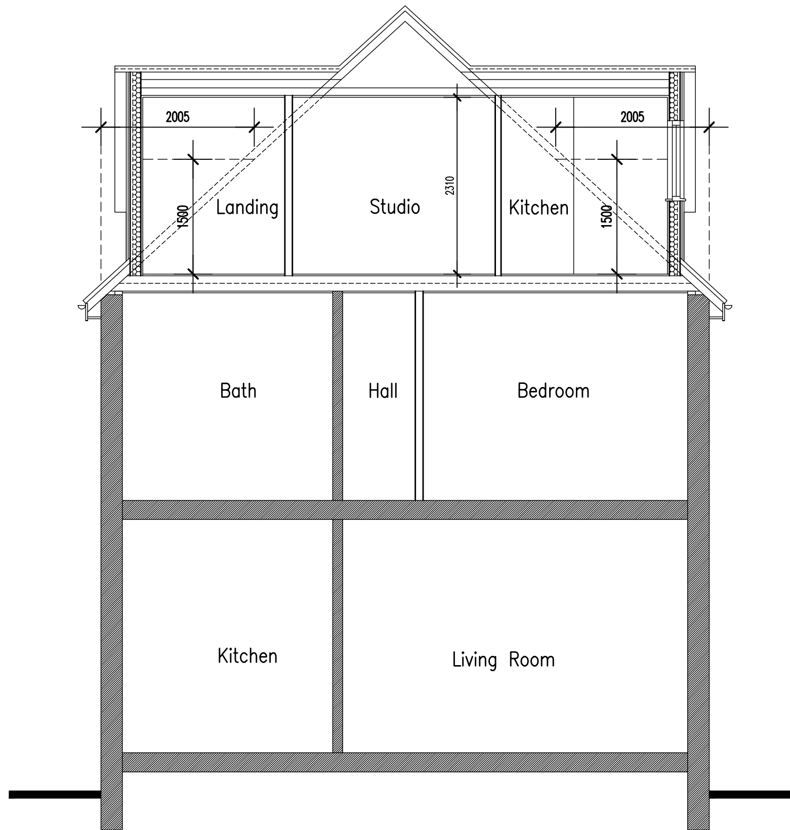
Typical Section
