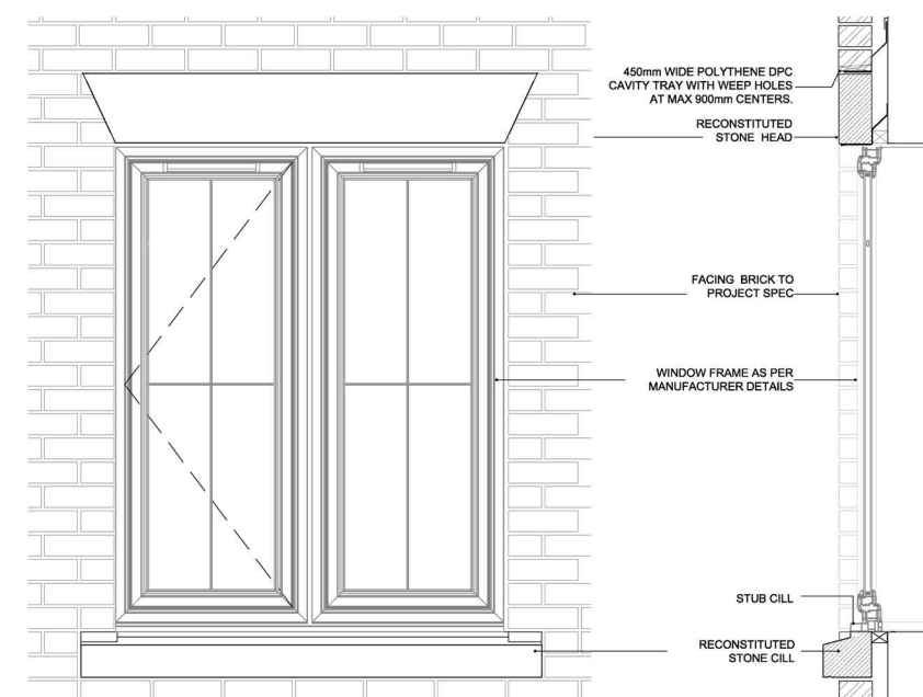
SPLAYED STONE HEADERS & STONE CILL WINDOW DETAILS TO PLOTS 25-30 & 36-45
