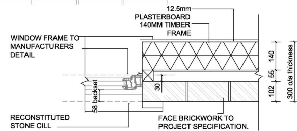
STONE HEADERS & CILL WINDOW DETAILS TO PLOTS 13, 17, 18, 21, 22, 31, 32, 34 & 35
