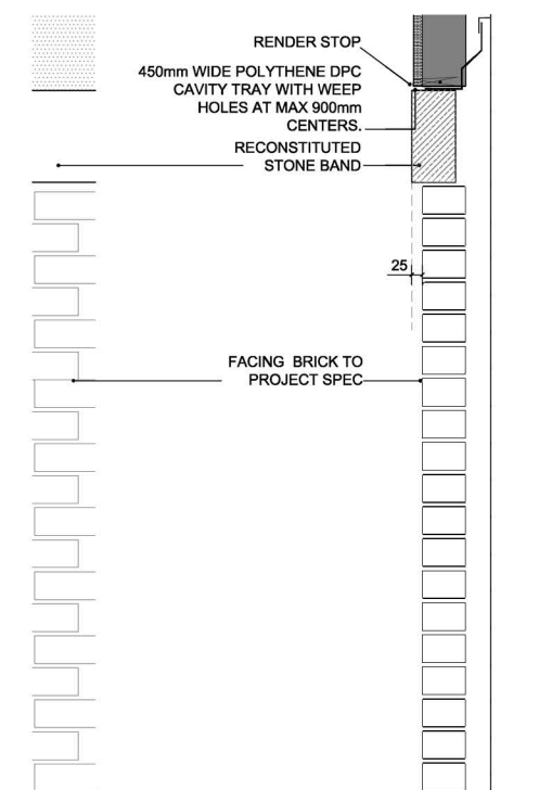
STONE BAND DETAIL TO PLOTS 25-30
