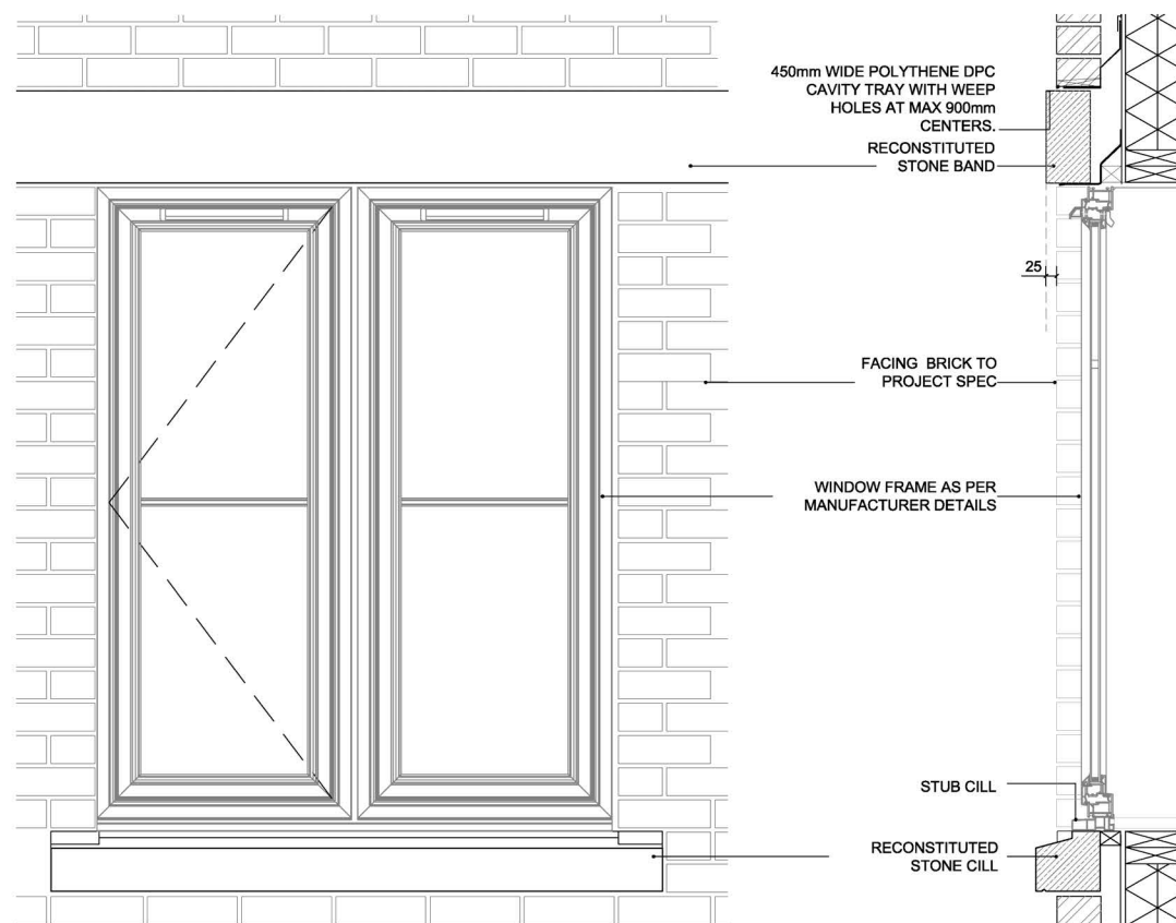
STONE BAND DETAIL TO PLOTS 25-30
