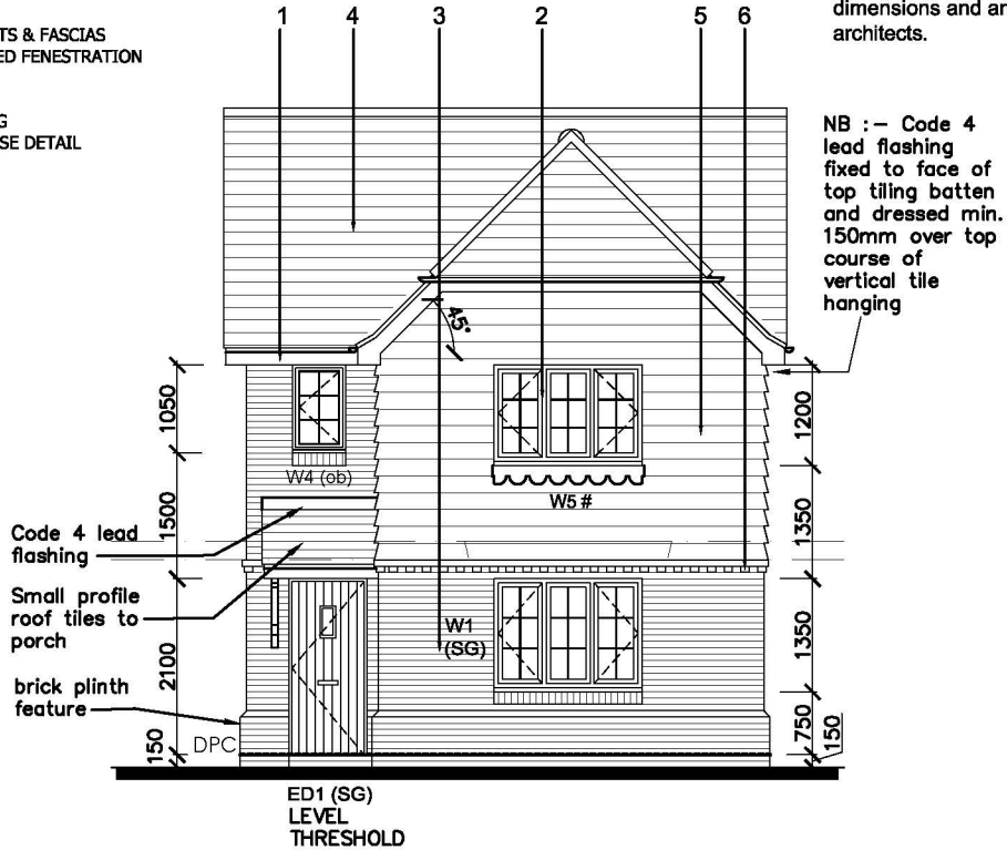
FRONT ELEVATION AS - Plot 6 1:100 scale OPP - Plot 5
