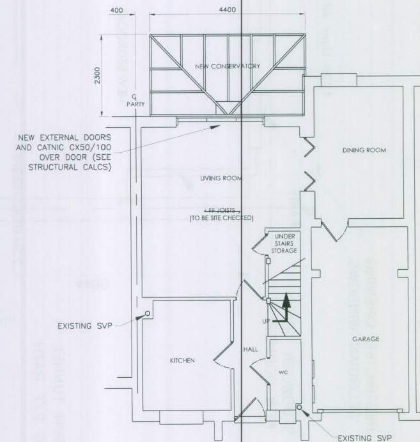
Proposed Ground
