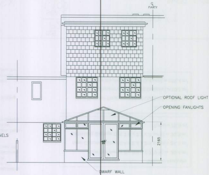
Proposed East Elevation (Rear) Indicative Conservatory Detail
