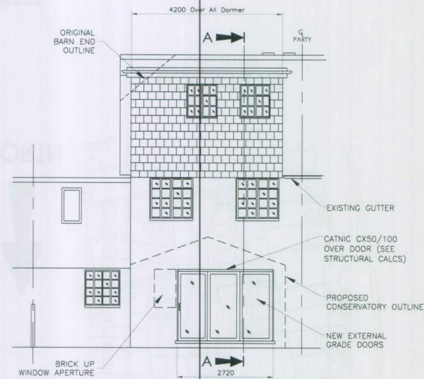
Proposed East Elevation (Rear) Showing Wall Modification
