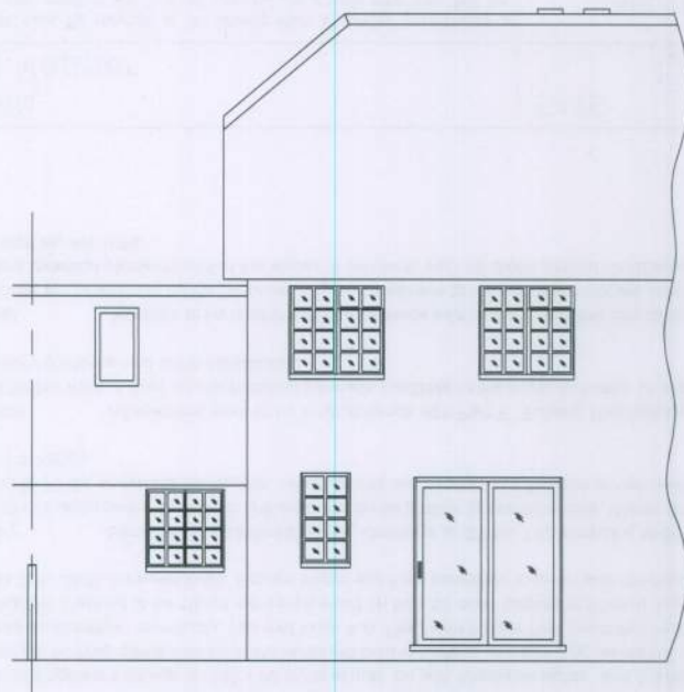
Existing East Elevation (Rear)
