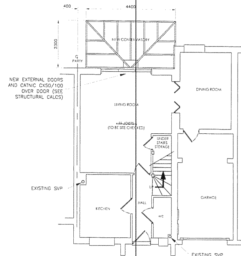
Proposed Ground
