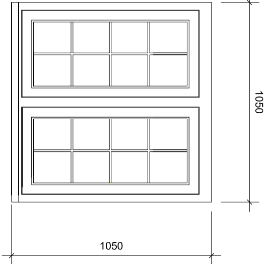
Window 9 & 10 Rear elevation
