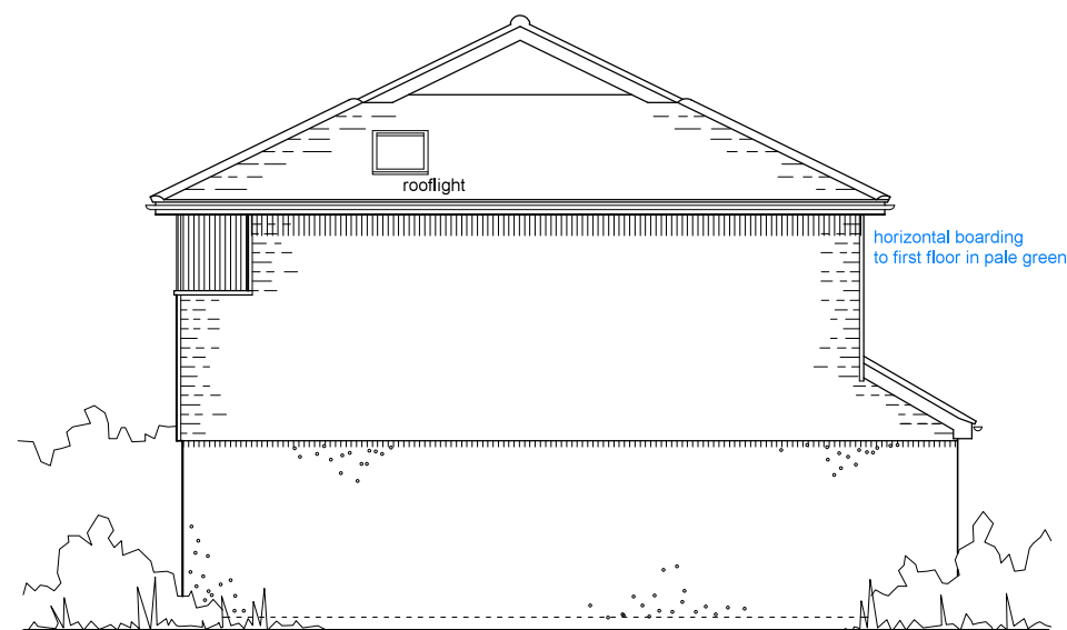
East Elevation
