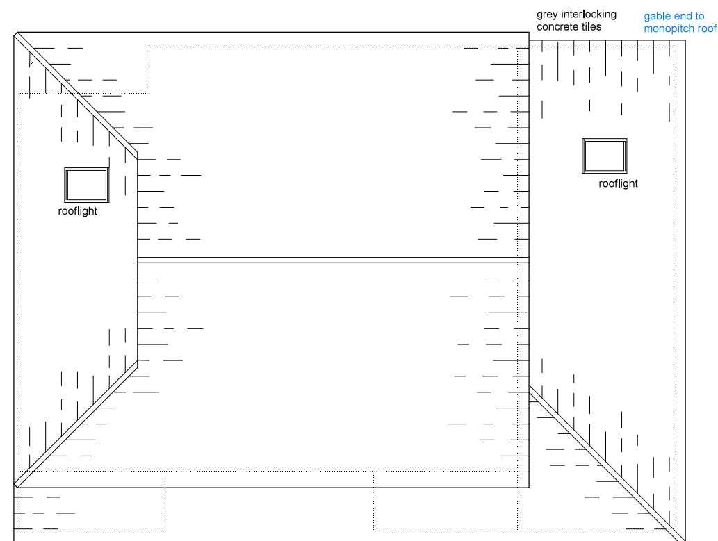
Roof Plan
