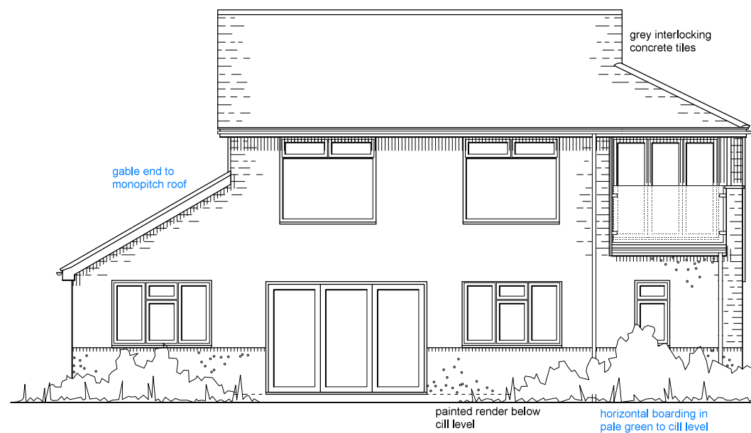
South Elevation
