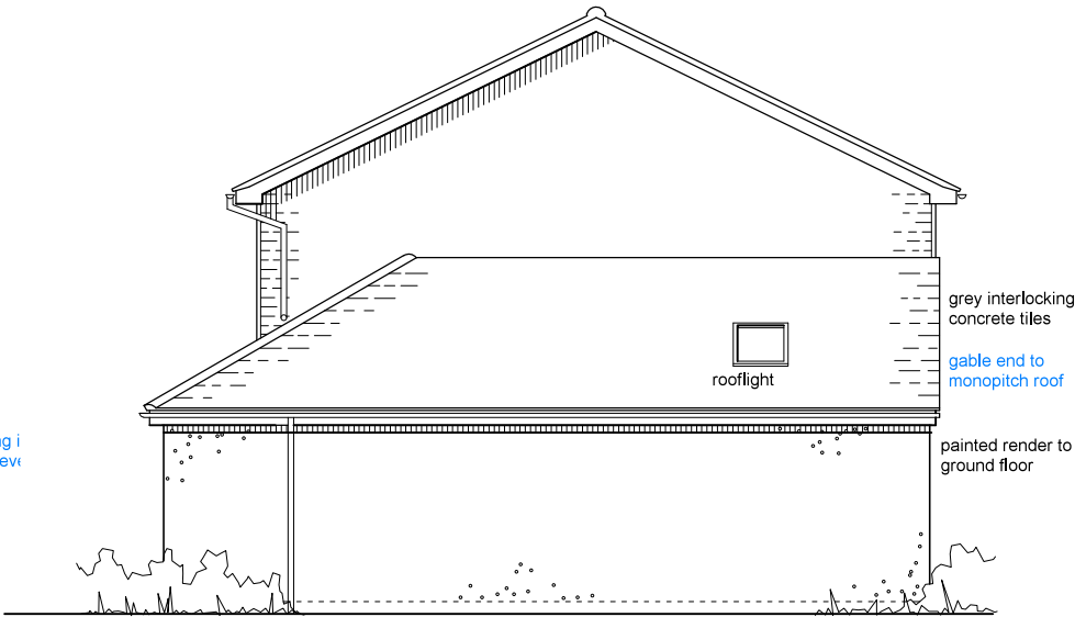
West Elevation
