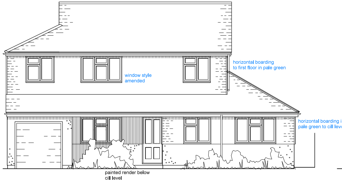
North Elevation
