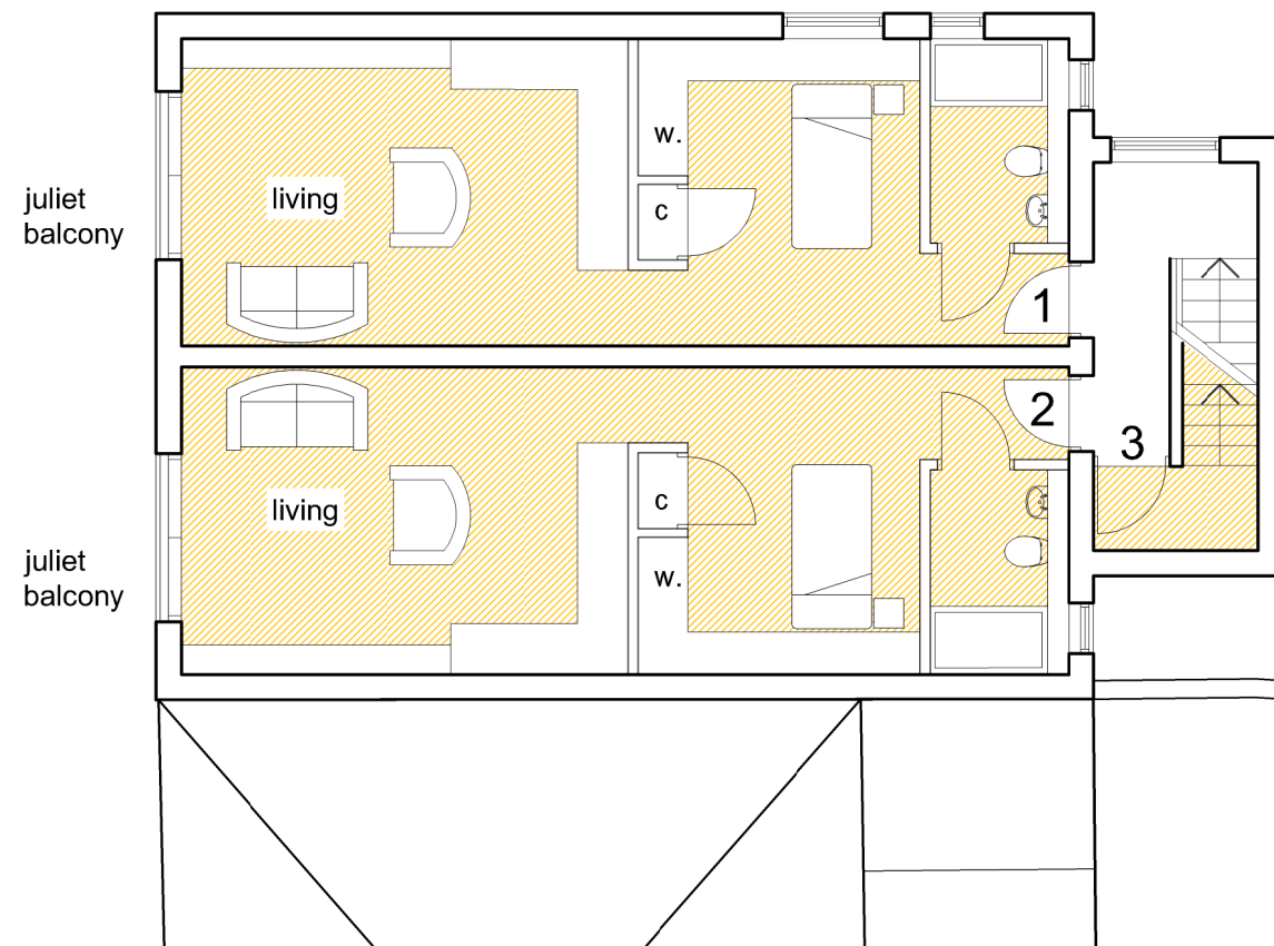
Proposed first floor plan Scale 1:100 @A3
