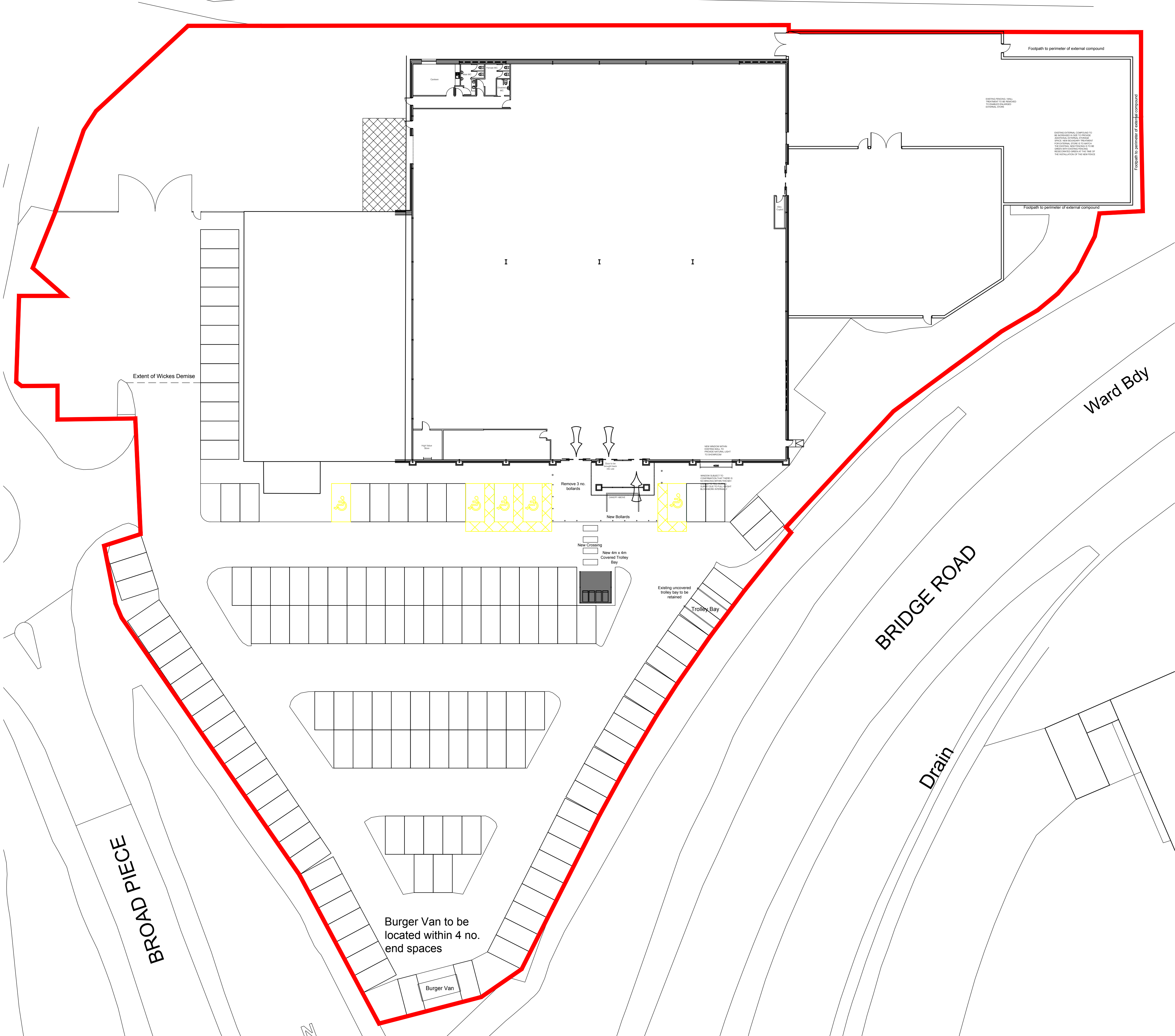
PROPOSED SITE LAYOUT PLAN SCALE - 1:250 AT A1
