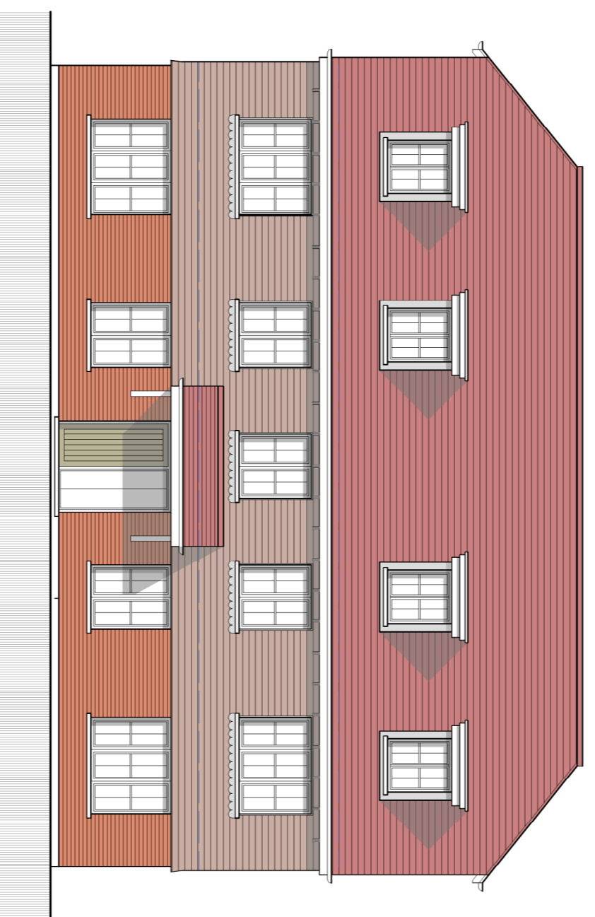
Proposed front / south elevation
