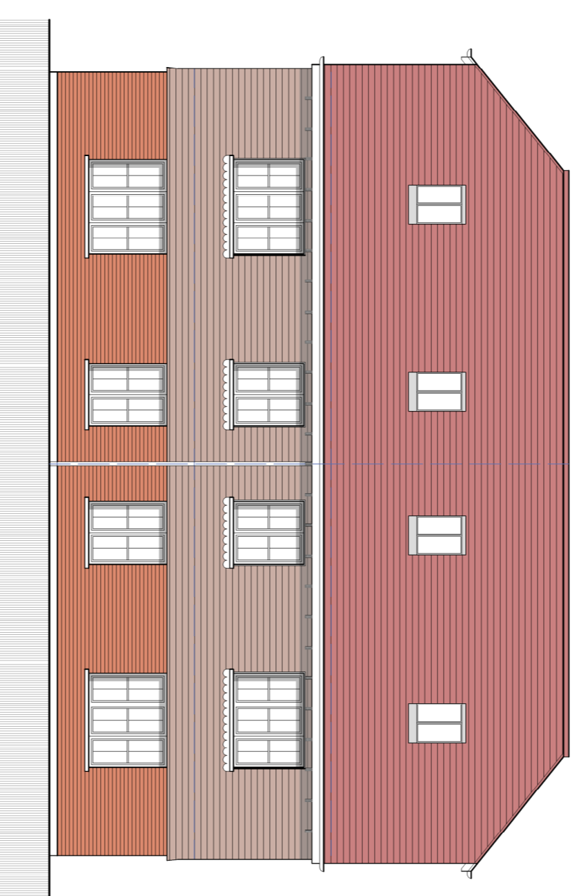
Proposed rear / north elevation
