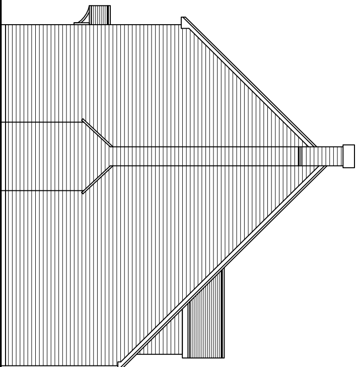
EXISTING WEST ELEVATION 1:100
