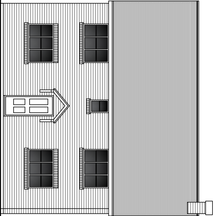
EXISTING NORTH ELEVATION 1:100
