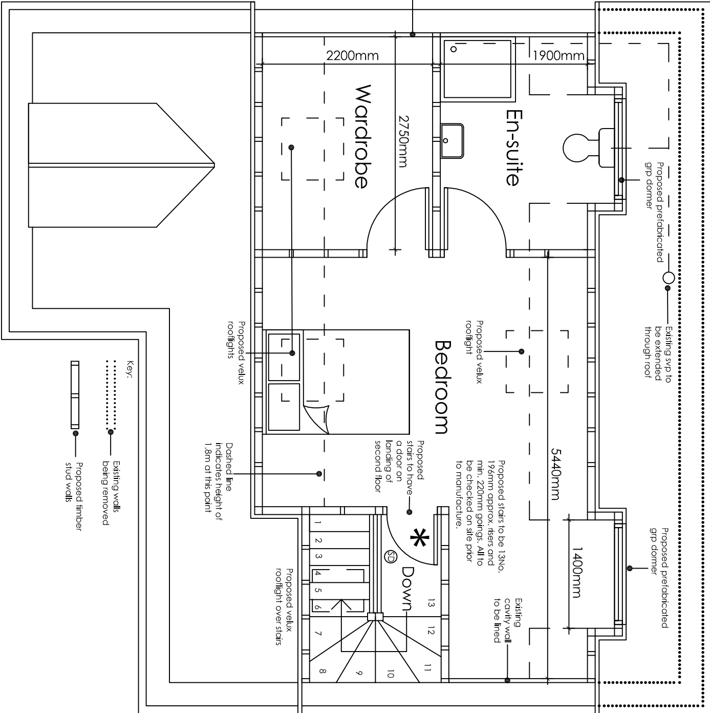
PROPOSED SECOND FLOOR PLAN 1:50
