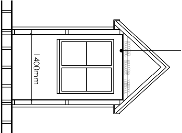
PROPOSED DORMER SECTION 1:50
