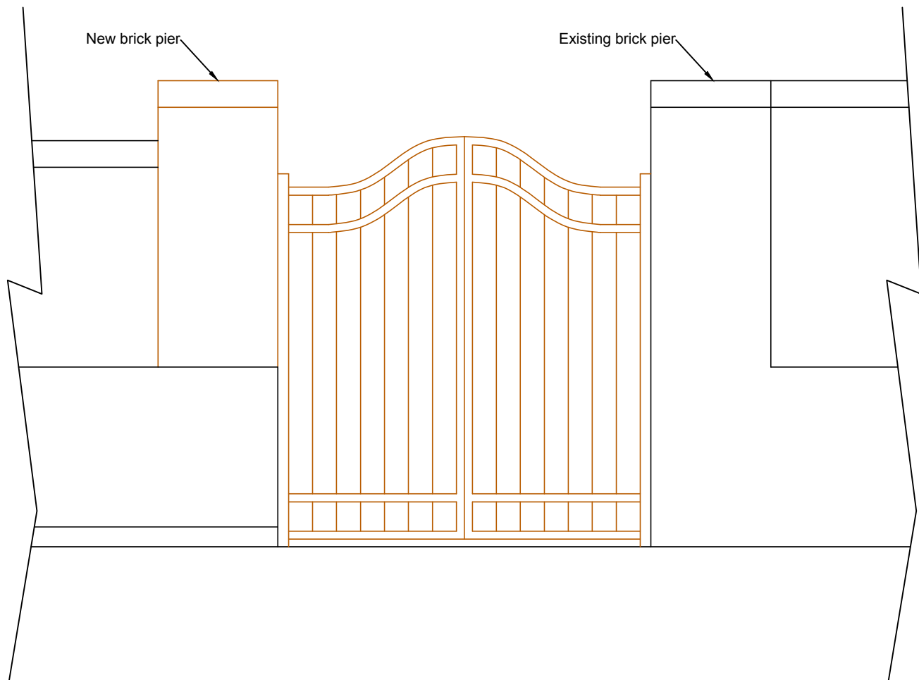
PROPOSED FRONT BOUNDARY WALL ELEVATION 1:20
