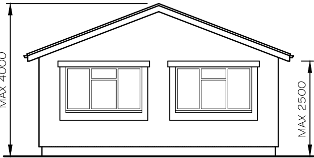
WEST ELEVATION
