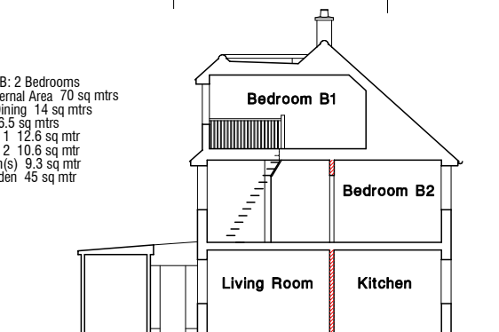
SECTION FACING EAST
