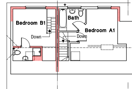
Proposed ATTIC PLAN
