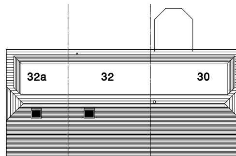
ROOF PLAN As Proposed 32a 32 30
