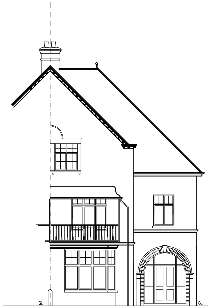
EXISTING FRONT (WEST) ELEVATION
