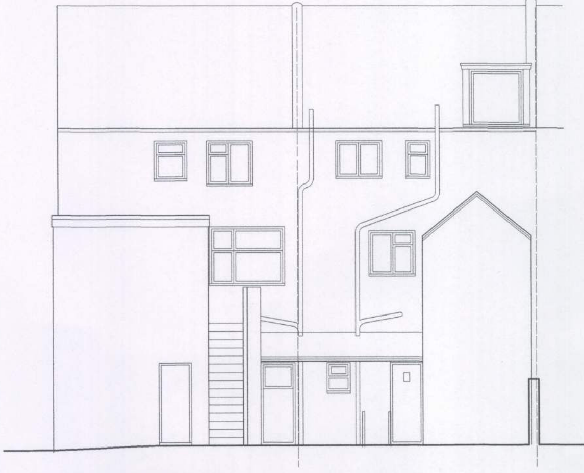
East Elevation to rear yard
