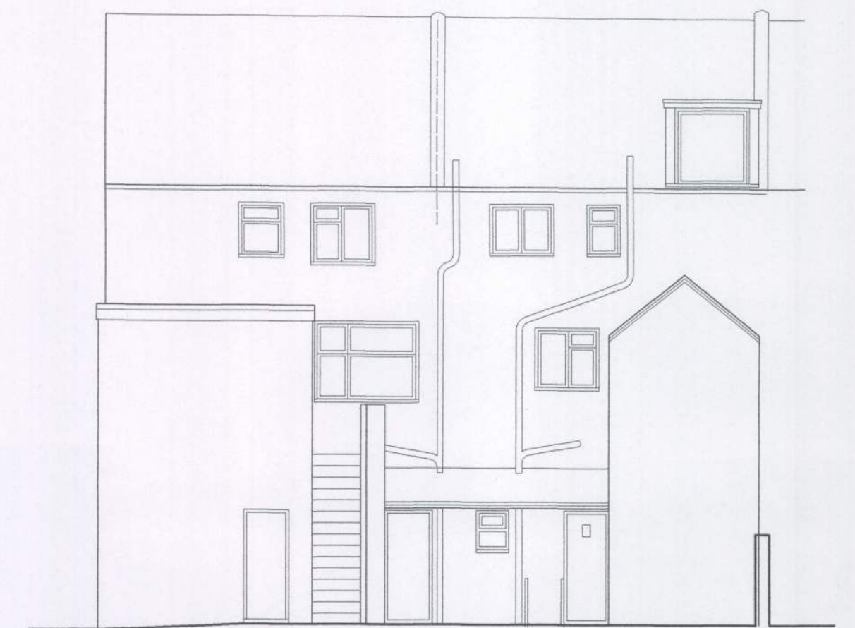
East Elevation to rear yard
